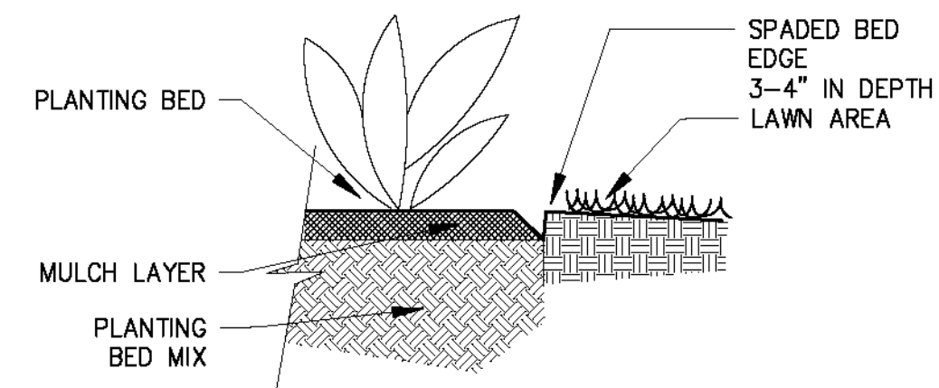
PLANTING BED EDGING Scale: 3/4" = 1'-0"
