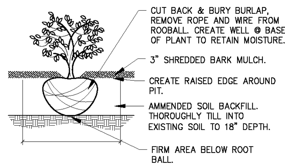
SHRUB PLANTING Scale: 3/4" = 1'-0"
