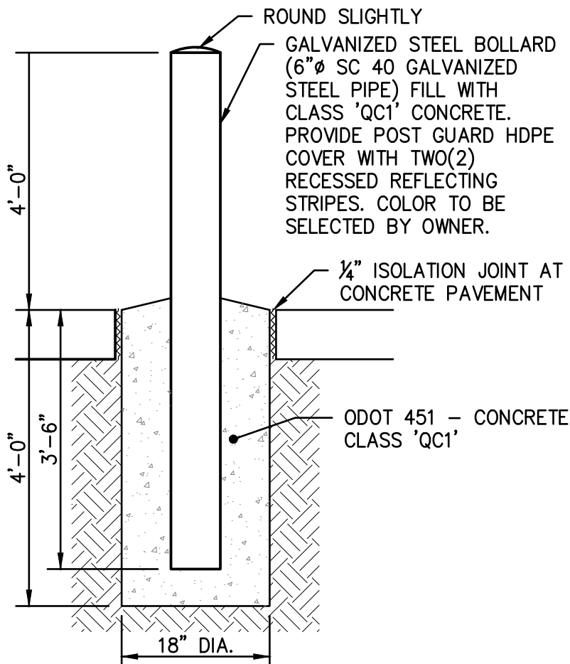
10 PIPE BOLLARD C5.00 NOT TO SCALE
