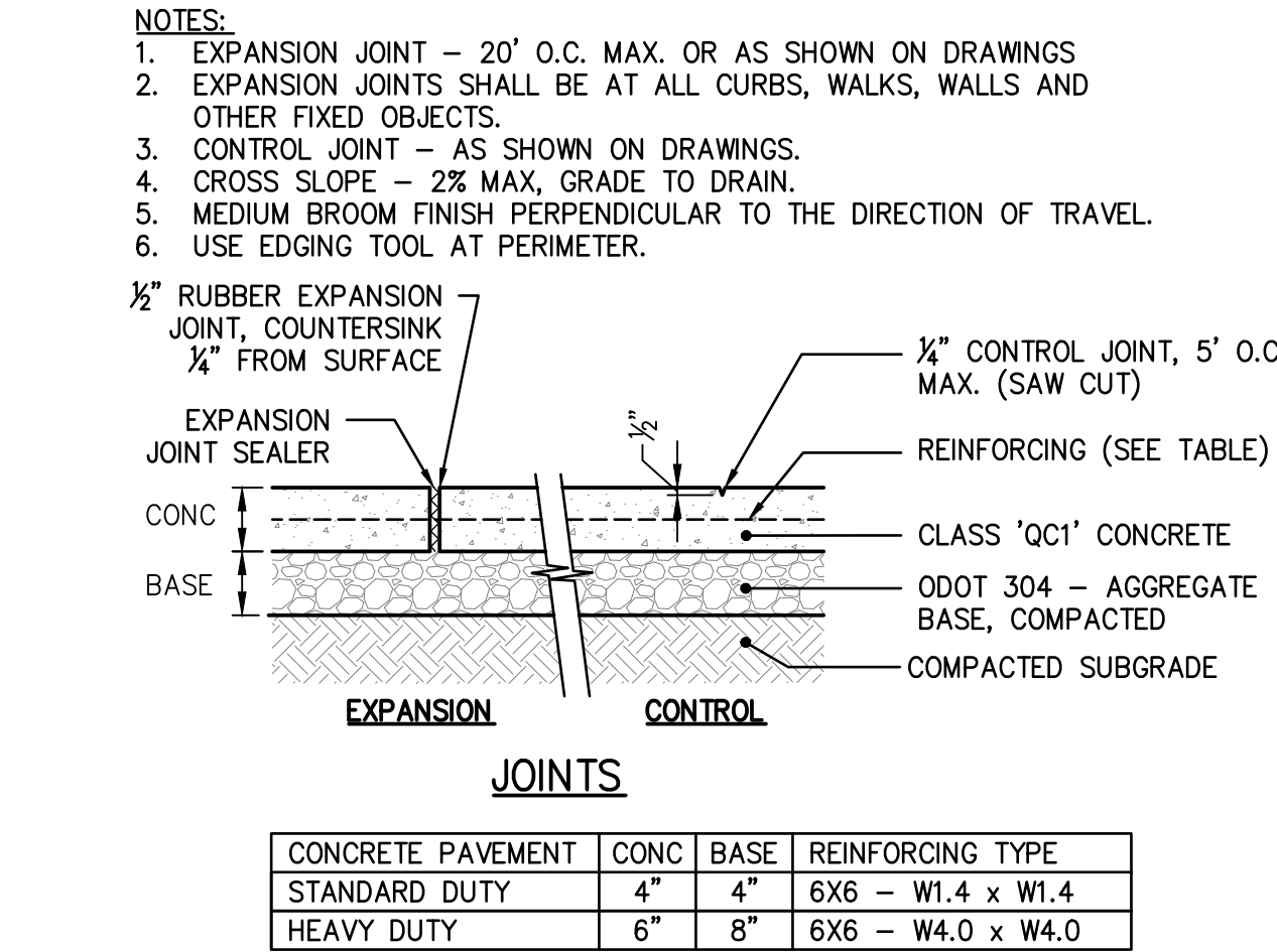
1 CONCRETE PAVEMENT C5.00 NOT TO SCALE
