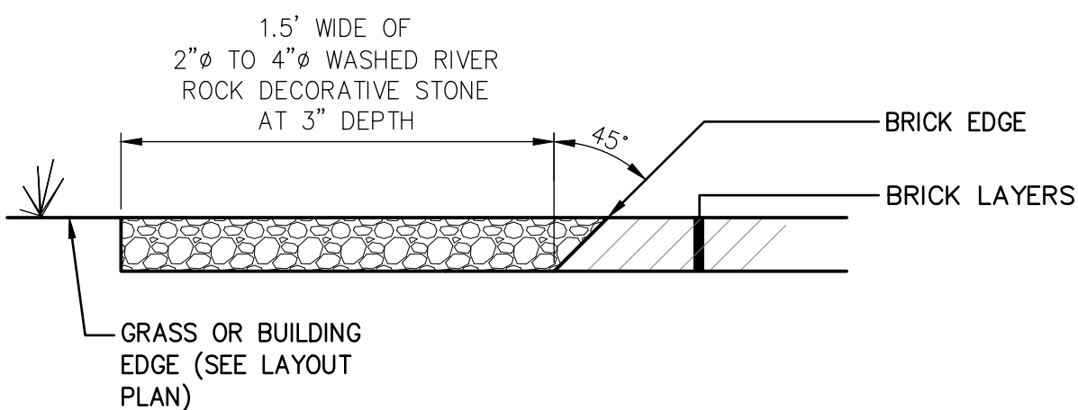
9 AGGREGATE SHOULDER C5.00 NOT TO SCALE
