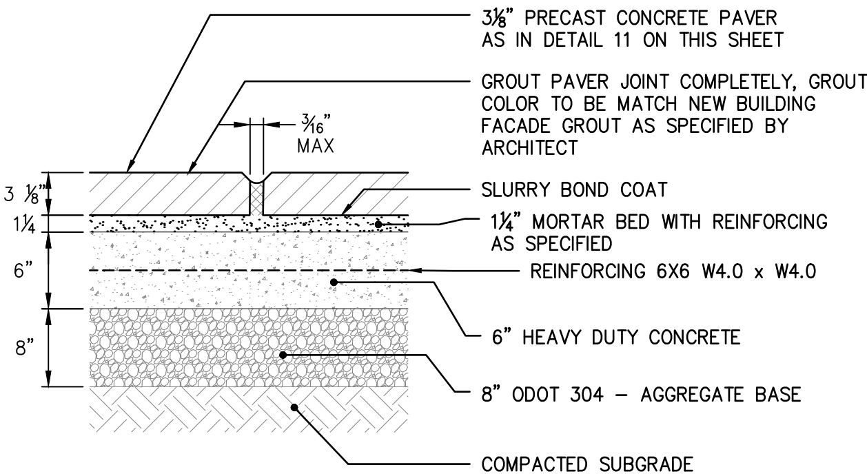
7 PRECAST DECORATIVE PAVER SETTING C5.00 NOT TO SCALE
