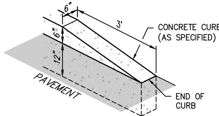
6 CURB END TAPER C5.00 NOT TO SCALE
