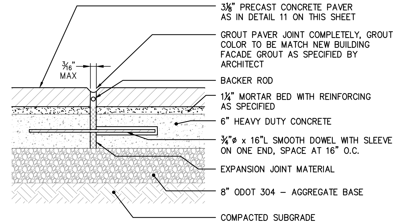
8 PRECAST DECORATIVE PAVER EXPANSION JOINT C5.00 NOT TO SCALE
