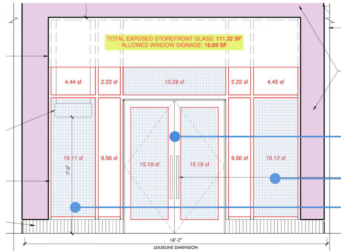
WINDOW DIMENSIONS
