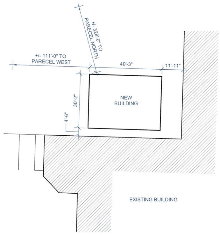
2 - ENLARGED SITE PLAN
