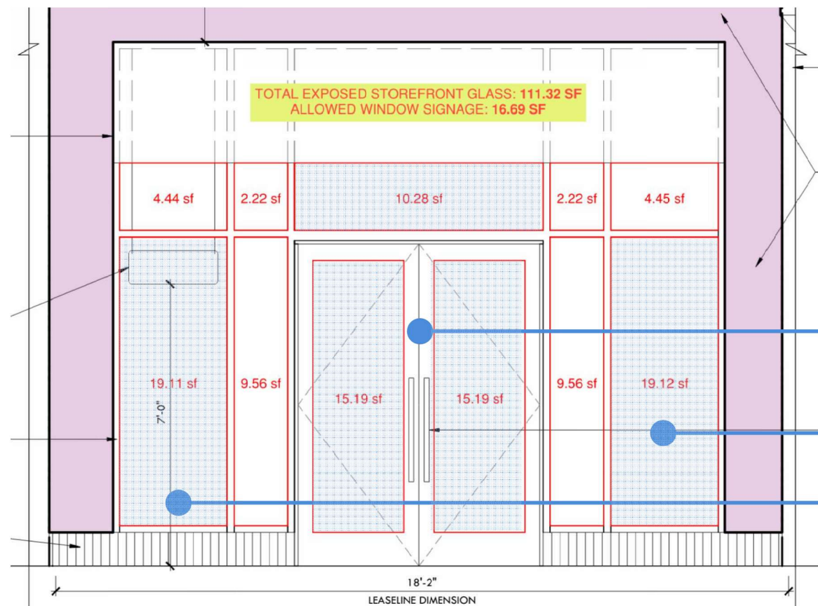
WINDOW DIMENSIONS
