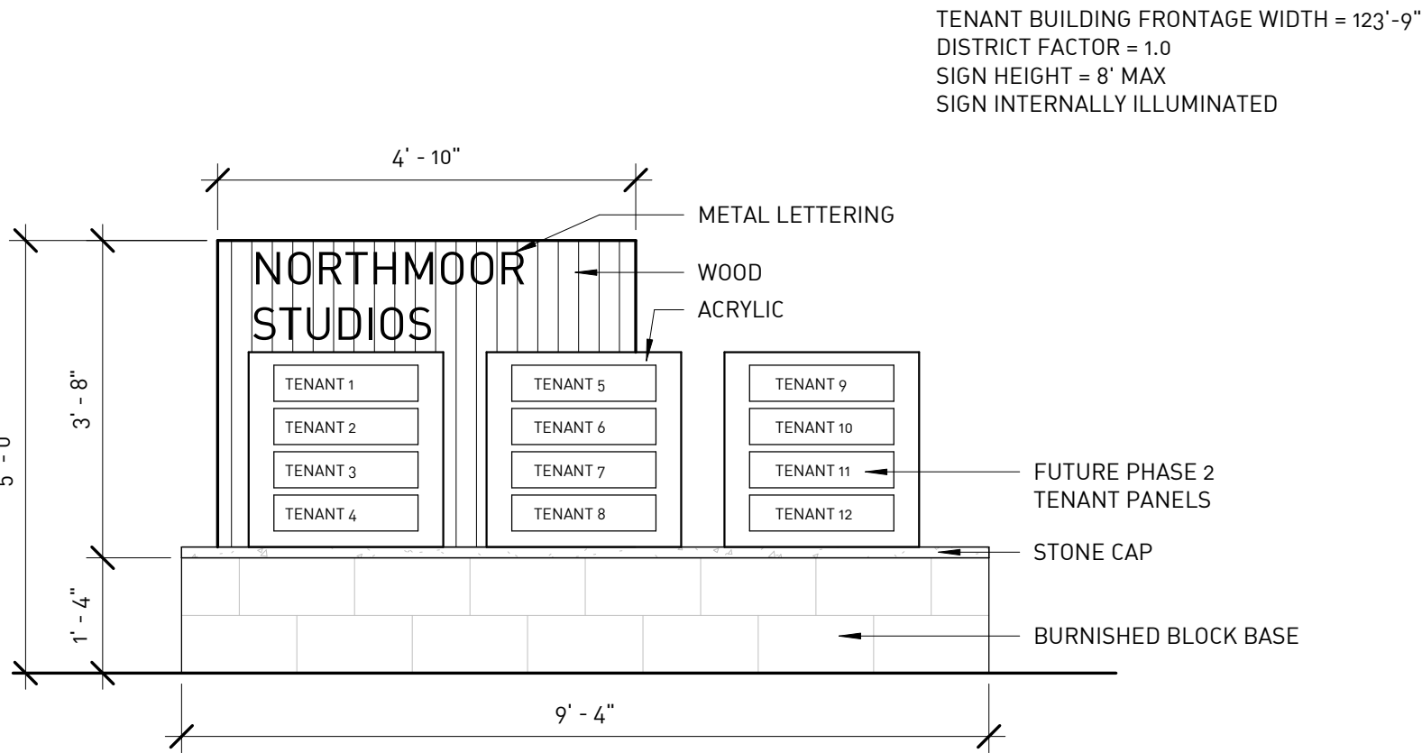
9 L401 MONUMENT SIGN - SITE 2 SCALE: 1/2" = 1'-0"
