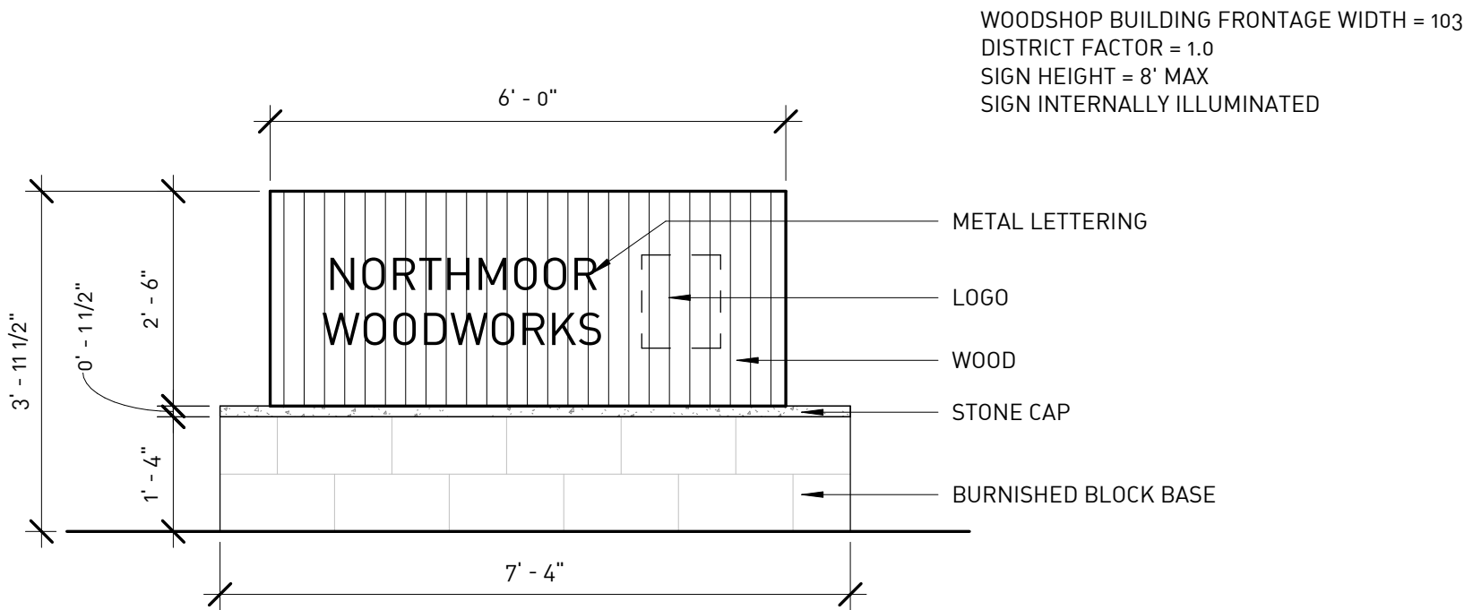
8 L401 MONUMENT SIGN - SITE 1 SCALE: 1/2" = 1'-0"
